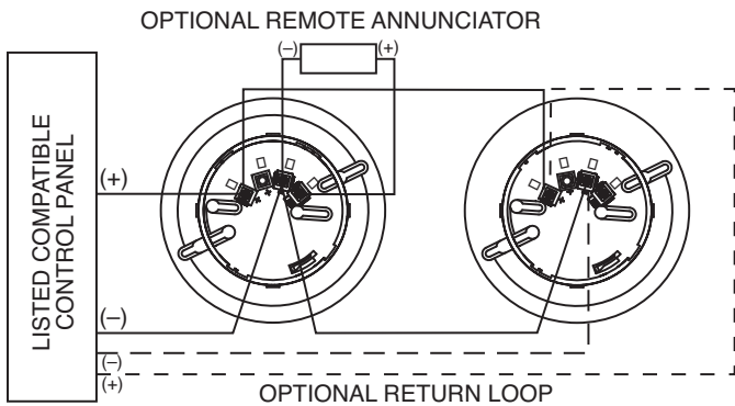
FIGURE 1. WIRING DIAGRAM:
