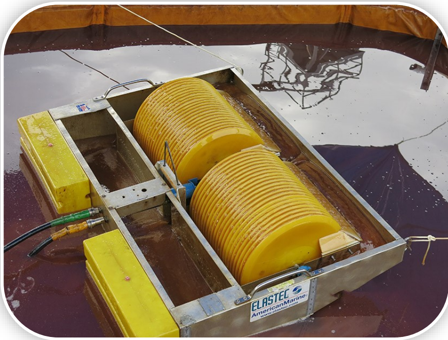
TDS118 Grooved Drum Skimmer
